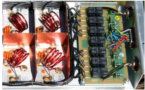
Figure 3 – Dunestar 600 RF Switching
